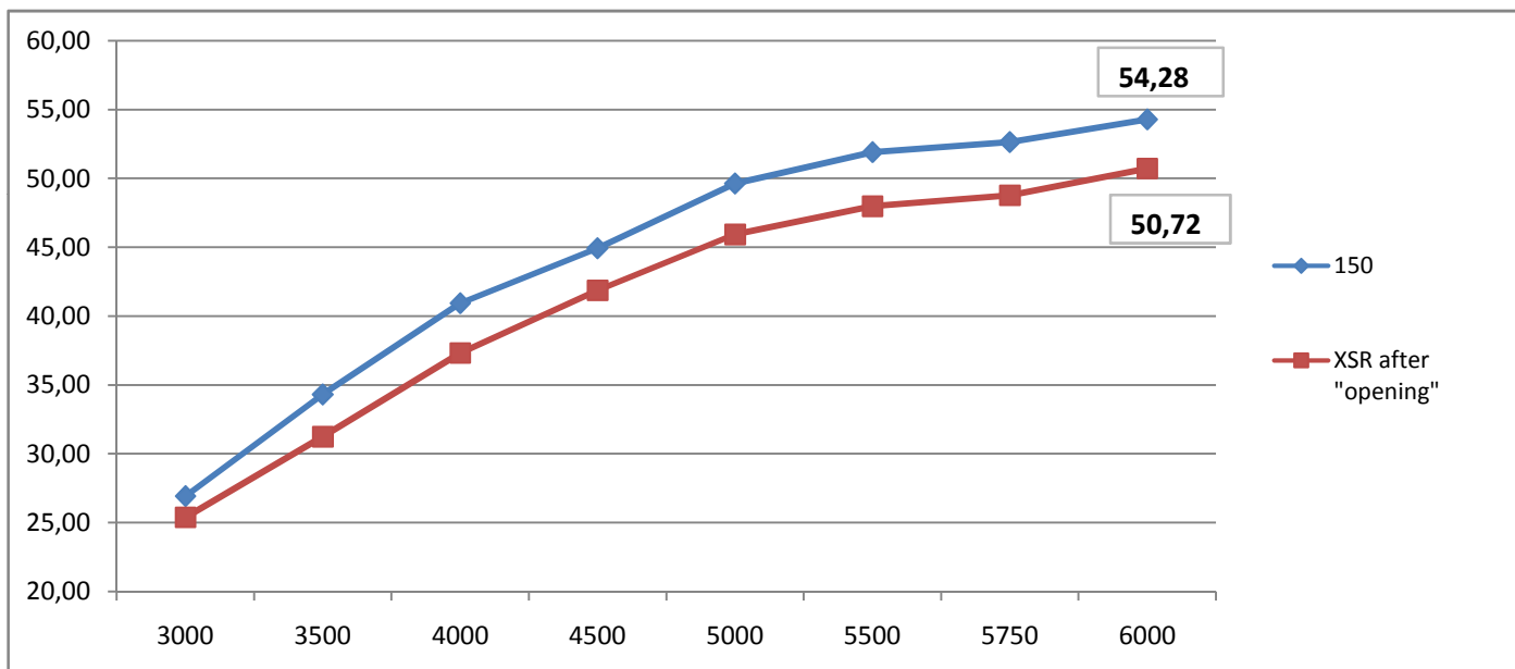
MAXIMUM FUEL CONSUMPTION (l/h)
