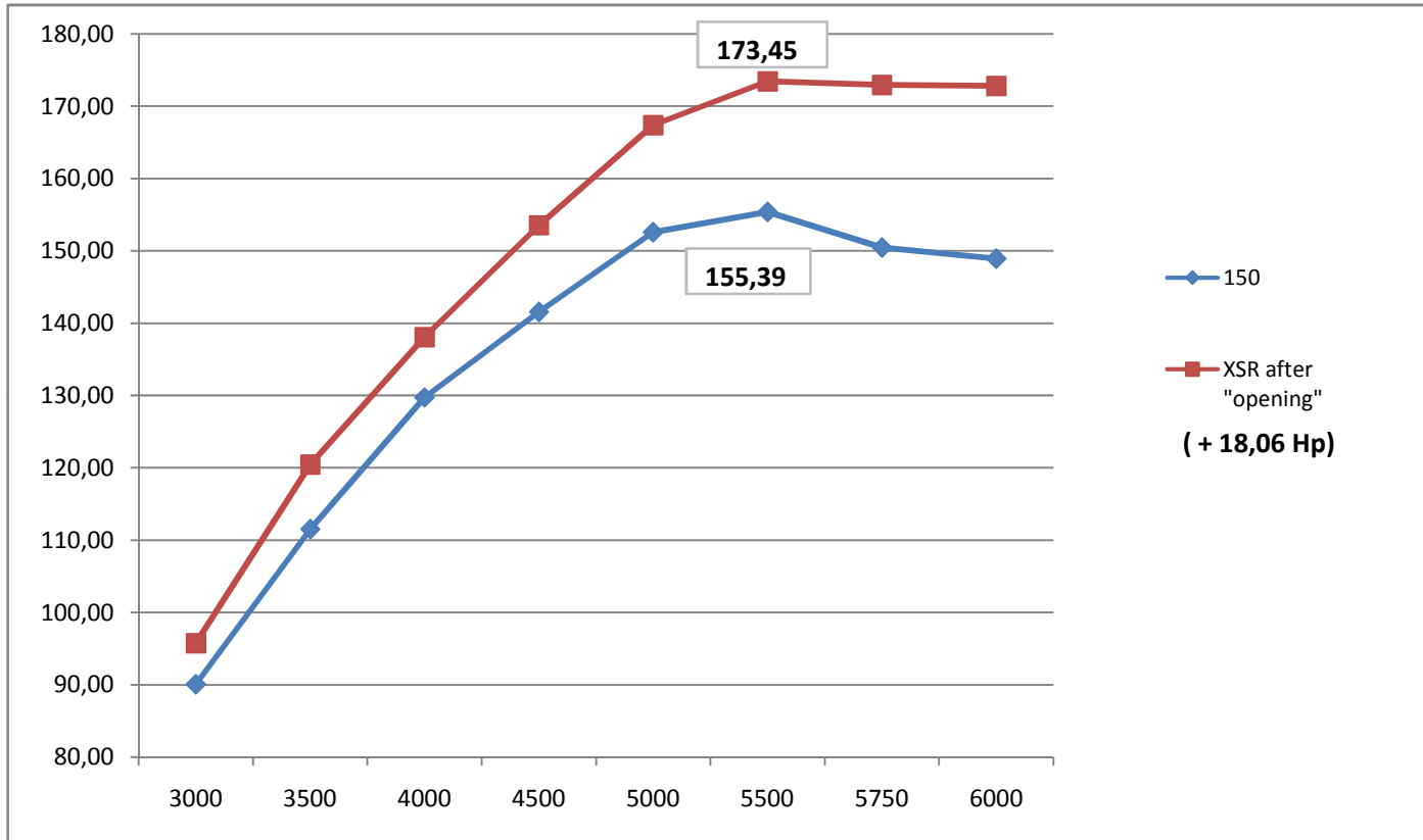
TORQUE AT THE PROPELLER SHAFT (Nm)
